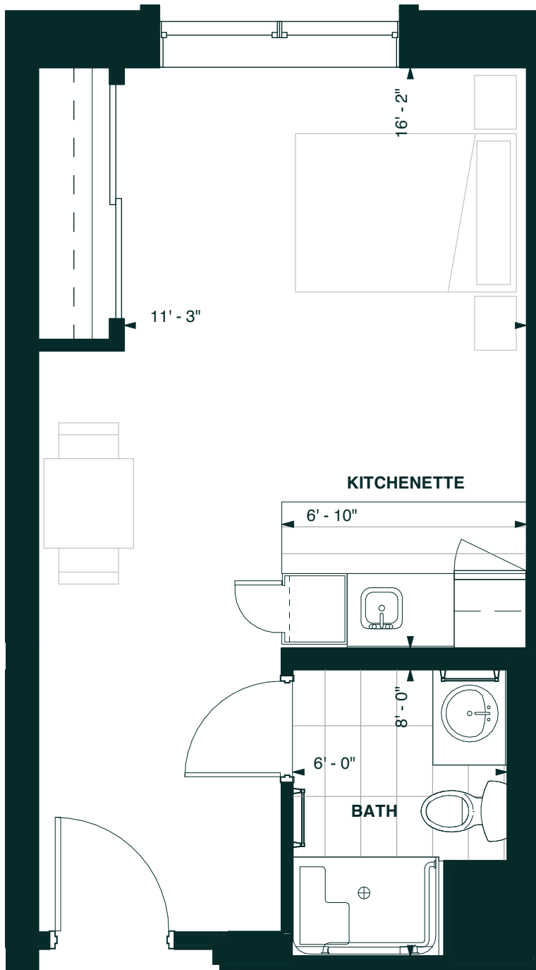
LAYOUT F Floors 1 & 3-6 ISL Studio Suite 381 SF
